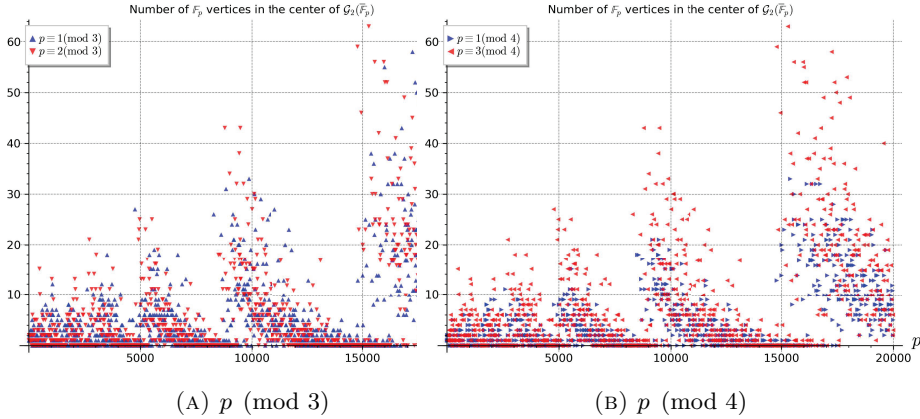
FIGURE 6.3. Number of \mathbb{F}_p -vertices in the center. Left: dark triangles pointing up (in blue), light triangles pointing down (in red) represent p \equiv 1 \pmod{3} , p \equiv 2 \pmod{3} (resp.). Right: dark triangles pointing right (in blue), light triangles pointing left (in red) represent p \equiv 1 \pmod{4} , p \equiv 3 \pmod{4} (resp.). COLOR ONLINE.
