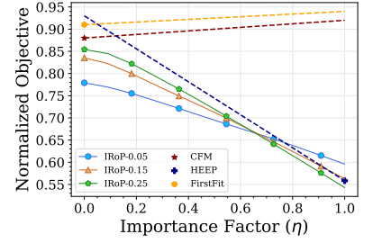
Fig. 6: Weighted sum of slowdown and energy of IRoP for different values of slowdown threshold compared to baselines.
