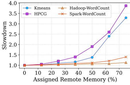
Fig. 2: Workload slowdown as the assigned remote memory ratio increases. The injected latency for remote memory is fixed at 5\mu s .
