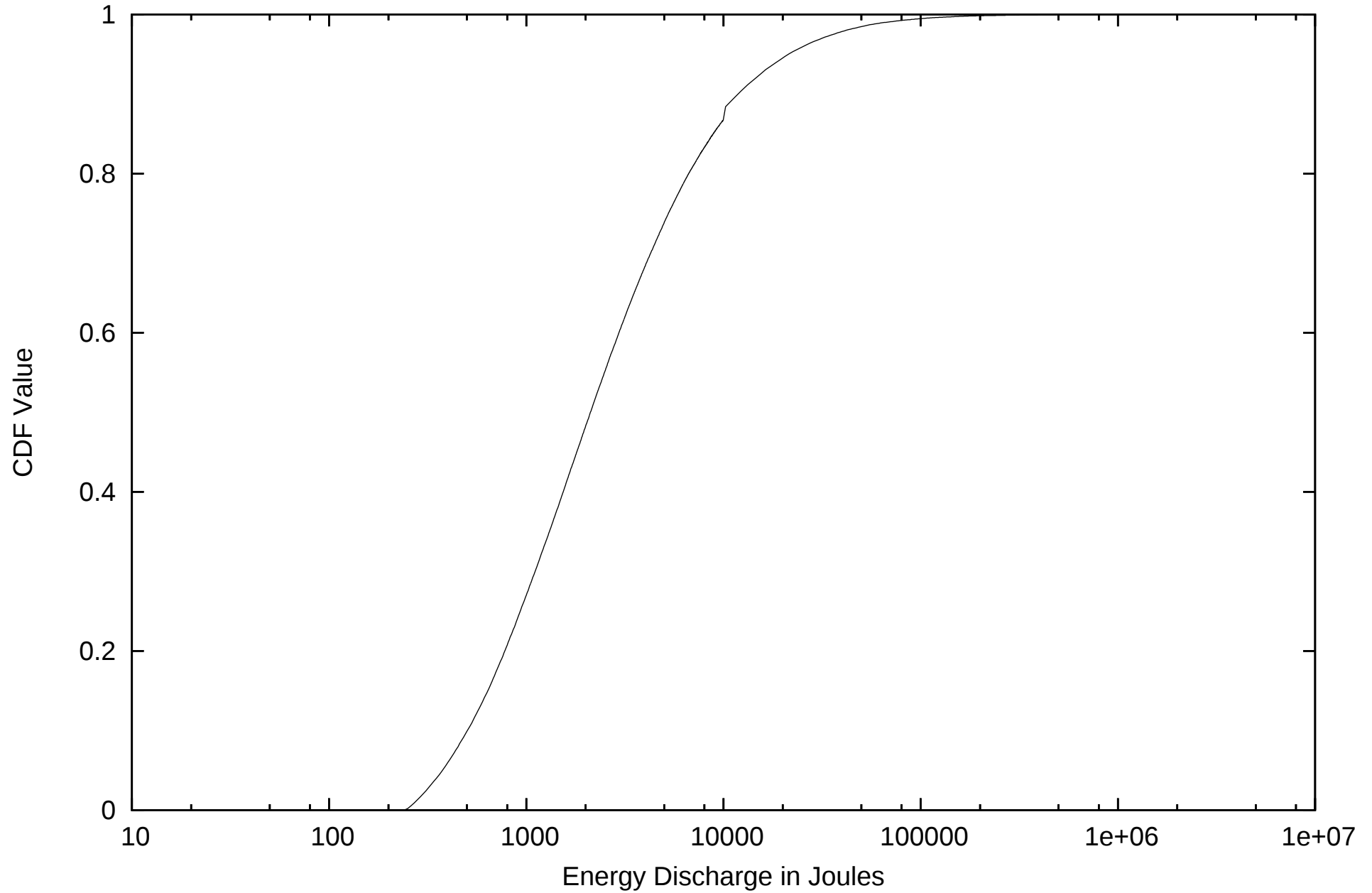
CDF of Energy Dissipation (Emperor)
